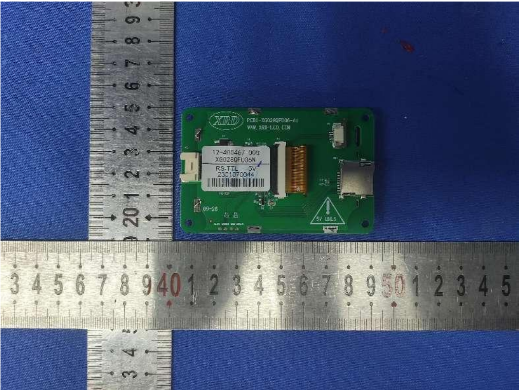
Fig.14---Bottom view of LCD PCB
