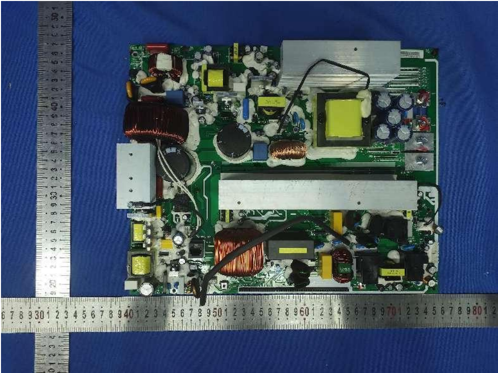
Fig.19---Top view of Main PCB
