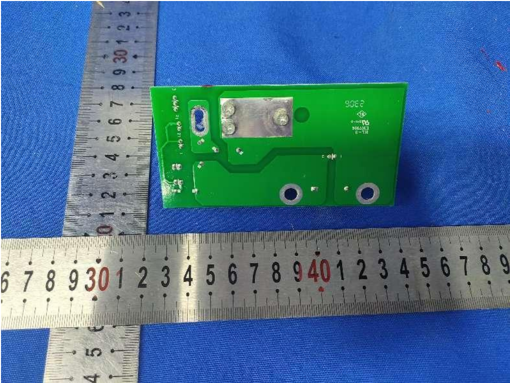
Fig.8---Bottom view of PCB
