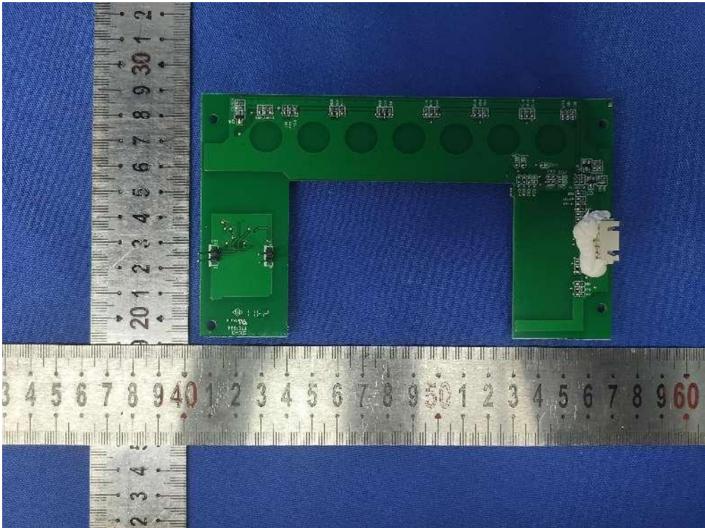
Fig.22---Bottom view of PCB
