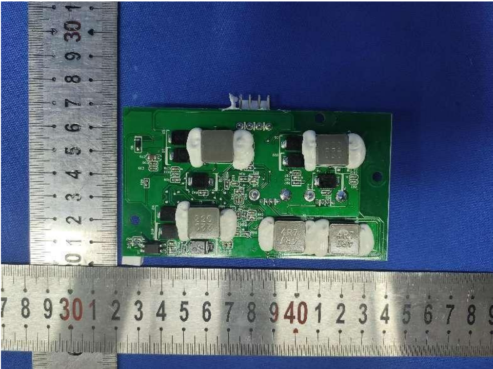
Fig.10--Bottom view of PCB
