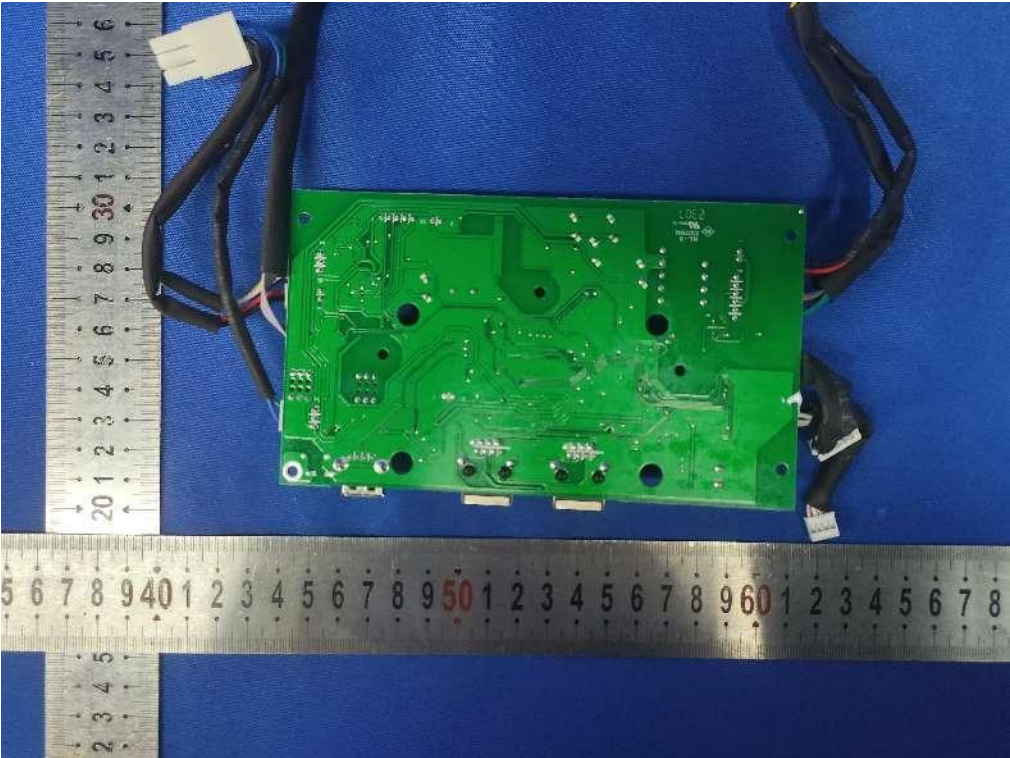
Fig.15---Top view of PCB
