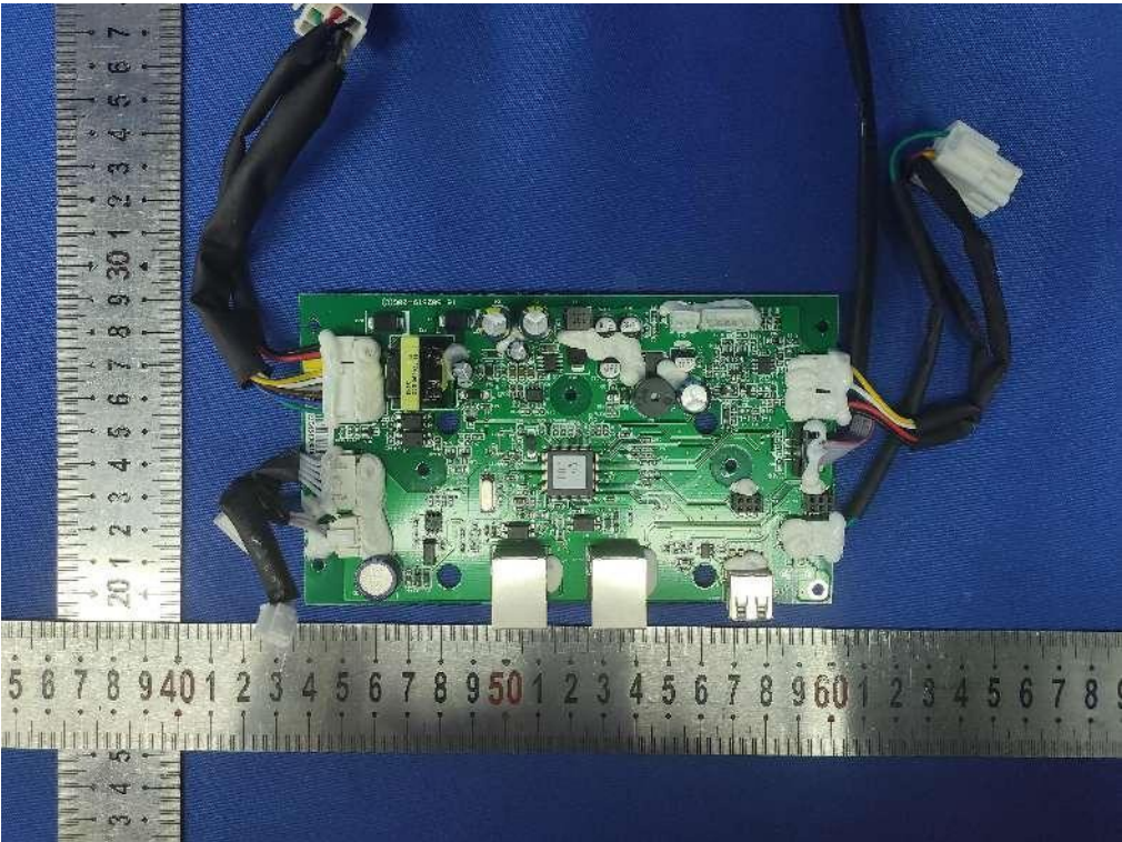
Fig.16---Bottom view of PCB
