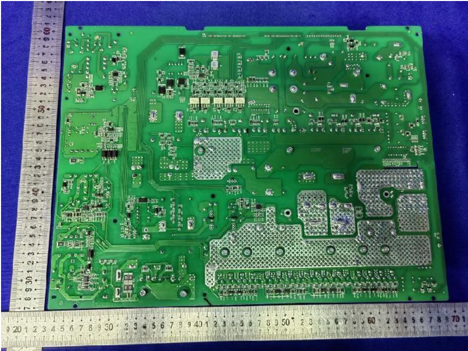
Fig. 6---PCB View
