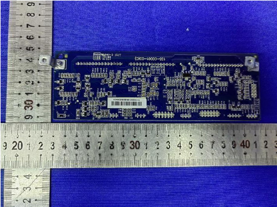
Fig. 12---PCB View
