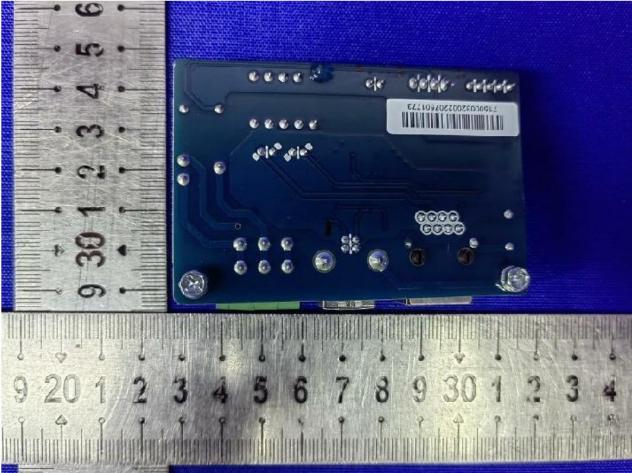
Fig. 8---PCB View
