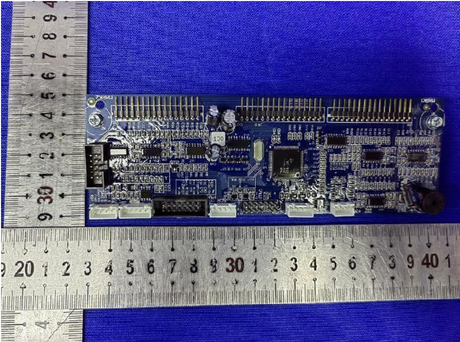
Fig. 11---PCB View
