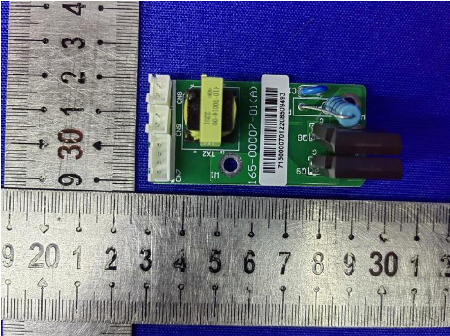
Fig. 13---PCB View
