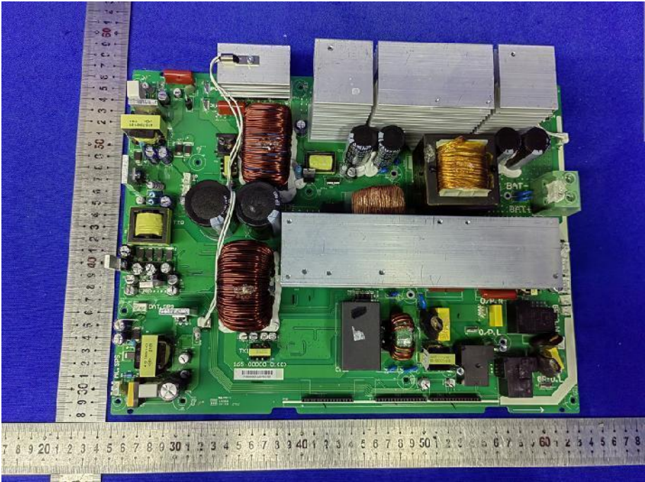
Fig. 5---PCB View
