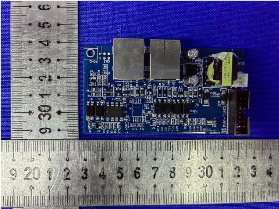
Fig. 9---PCB View
