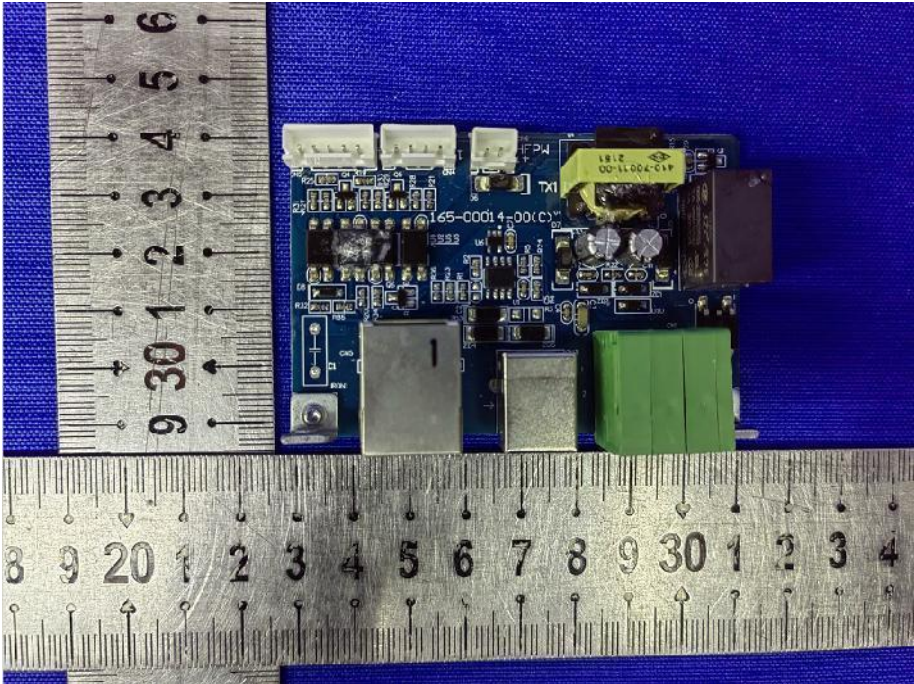
Fig. 7---PCB View
