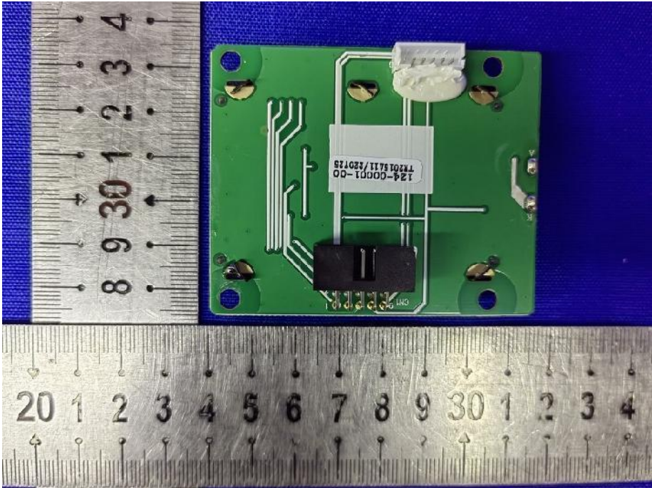
Fig. 18---PCB View
