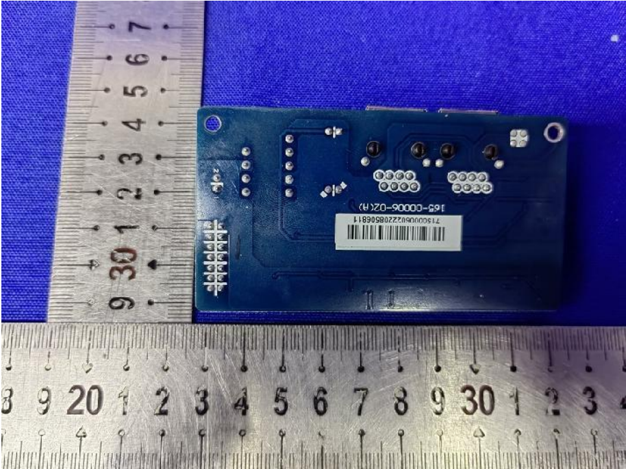
Fig. 10---PCB View
