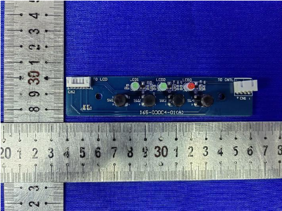
Fig. 15---PCB View
