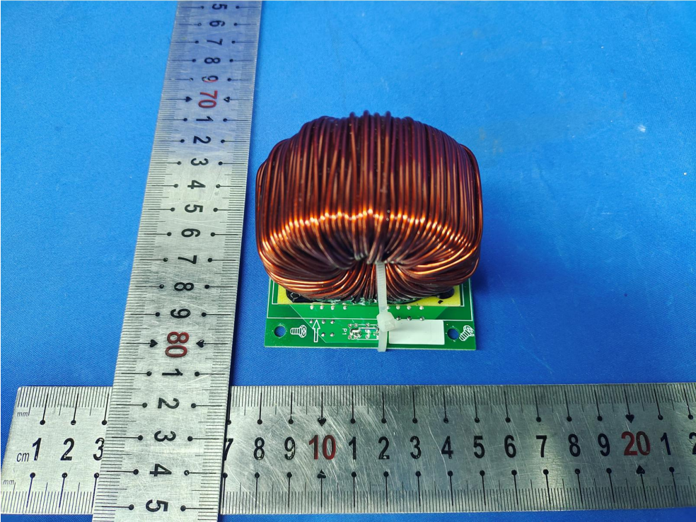
Fig. 22---PCB View
