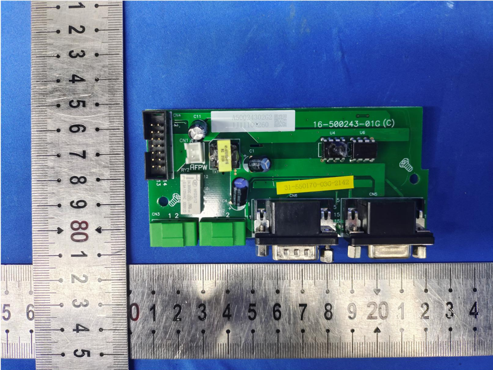
Fig. 14---PCB View
