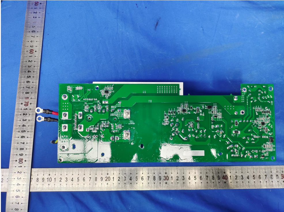
Fig. 11---PCB View
