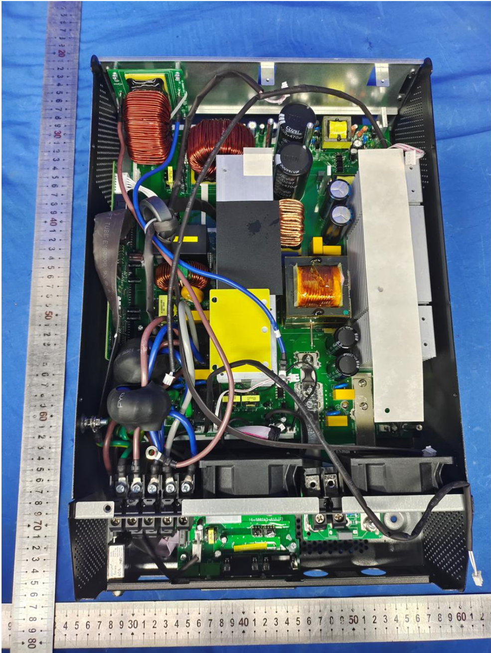
Fig. 7---Internal View
