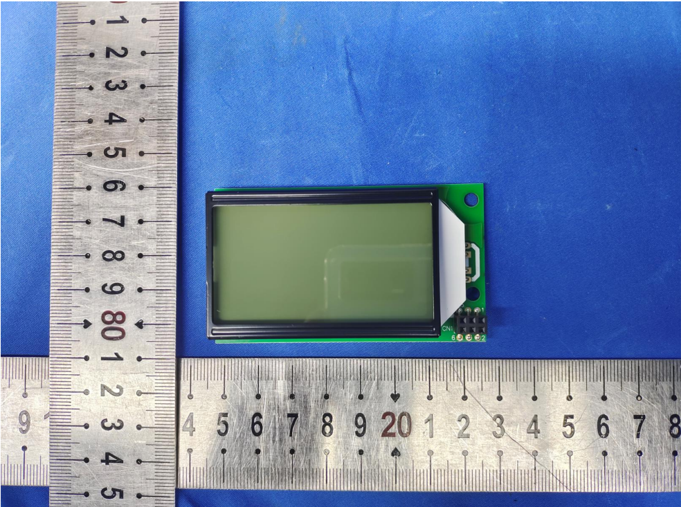
Fig. 20---PCB View
