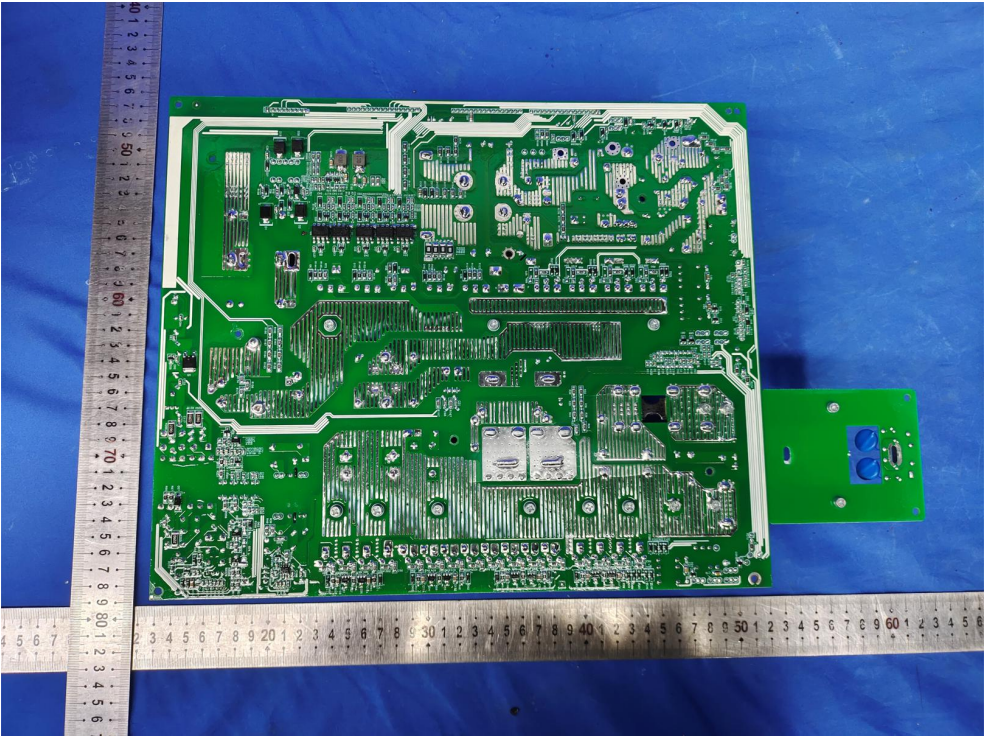
Fig. 9---PCB View
