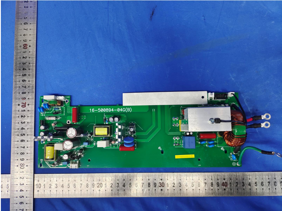
Fig. 10---PCB View
