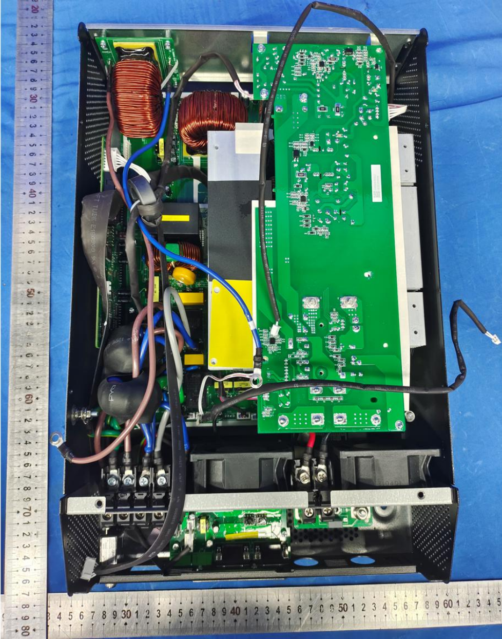
Fig. 6---Internal View
