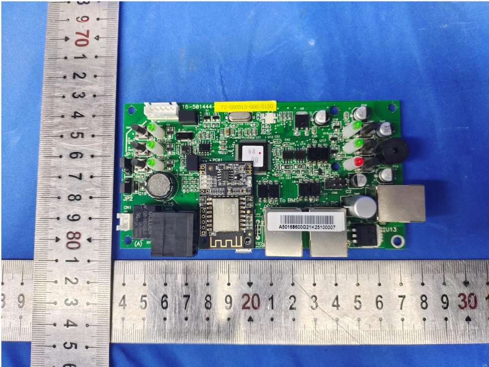
Fig. 18---PCB View
