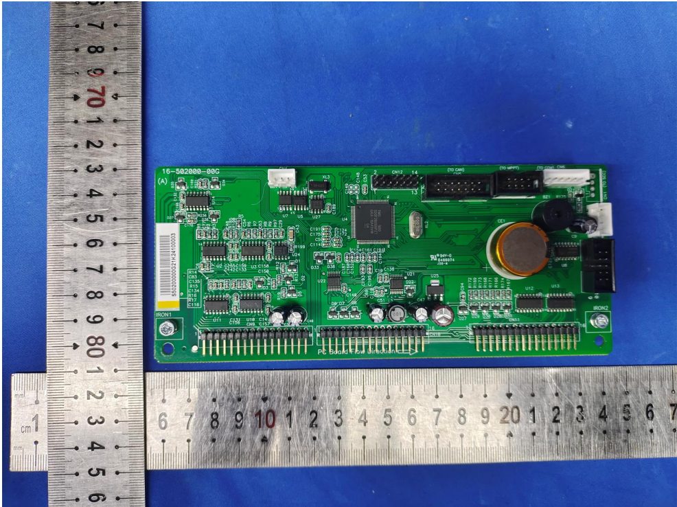
Fig. 12---PCB View
