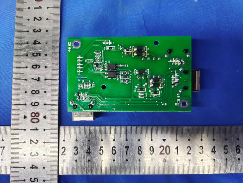
Fig. 17---PCB View
