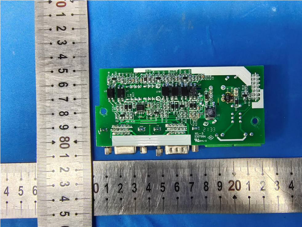
Fig. 15---PCB View
