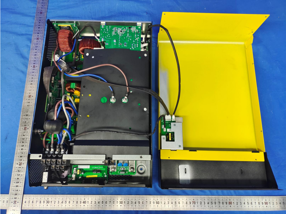
Fig. 5--- Internal View
