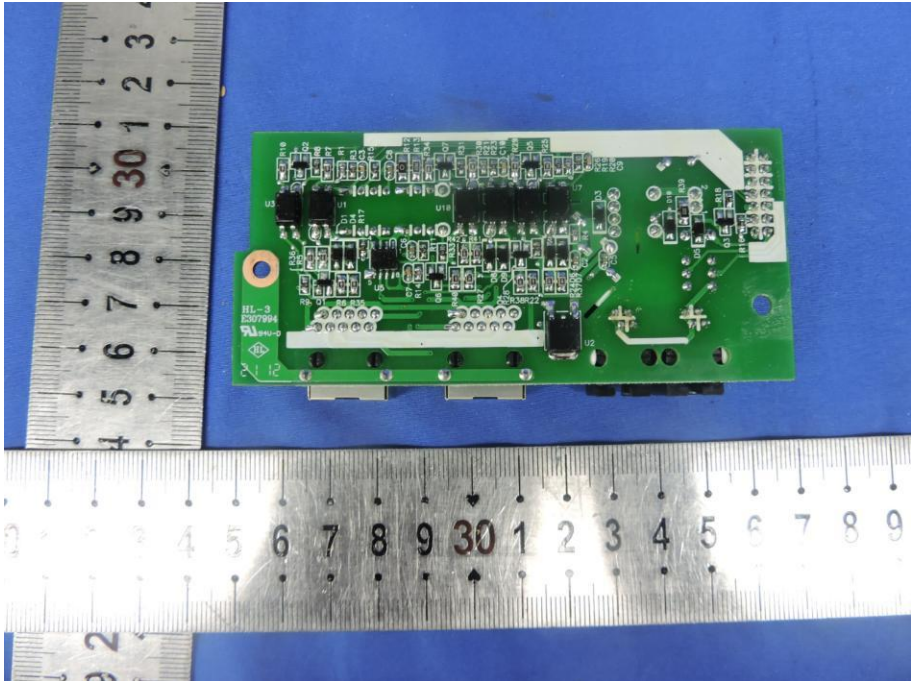
Fig. 30---PCB View
