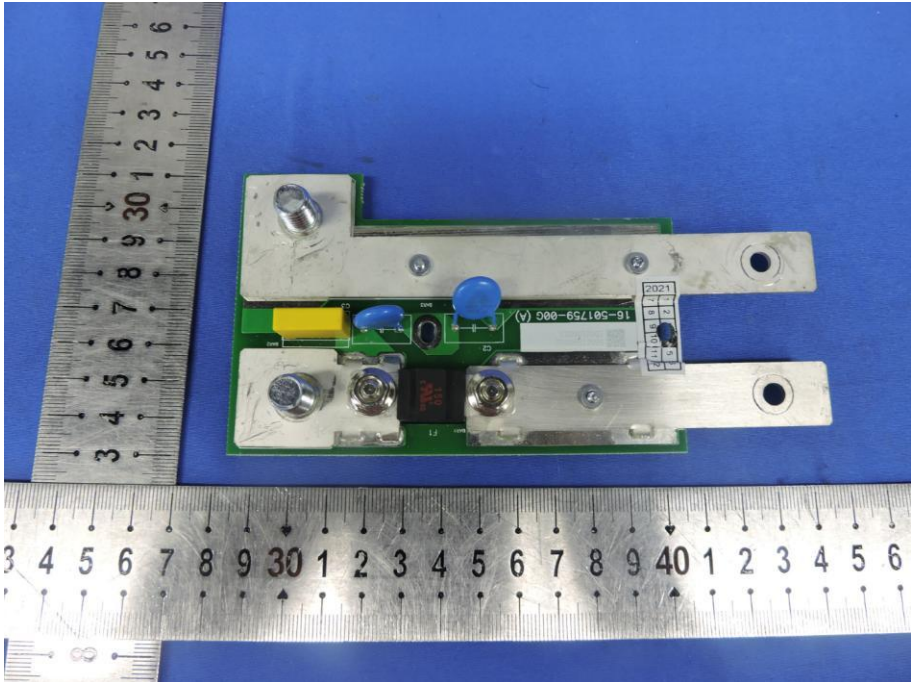
Fig. 23---PCB View
