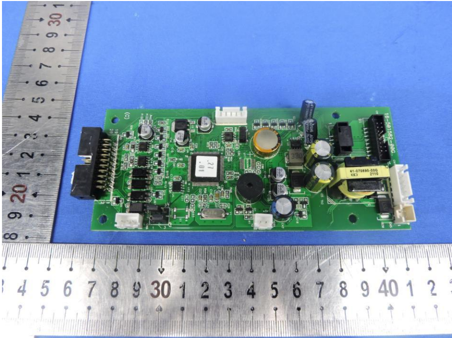
Fig. 15---PCB View
