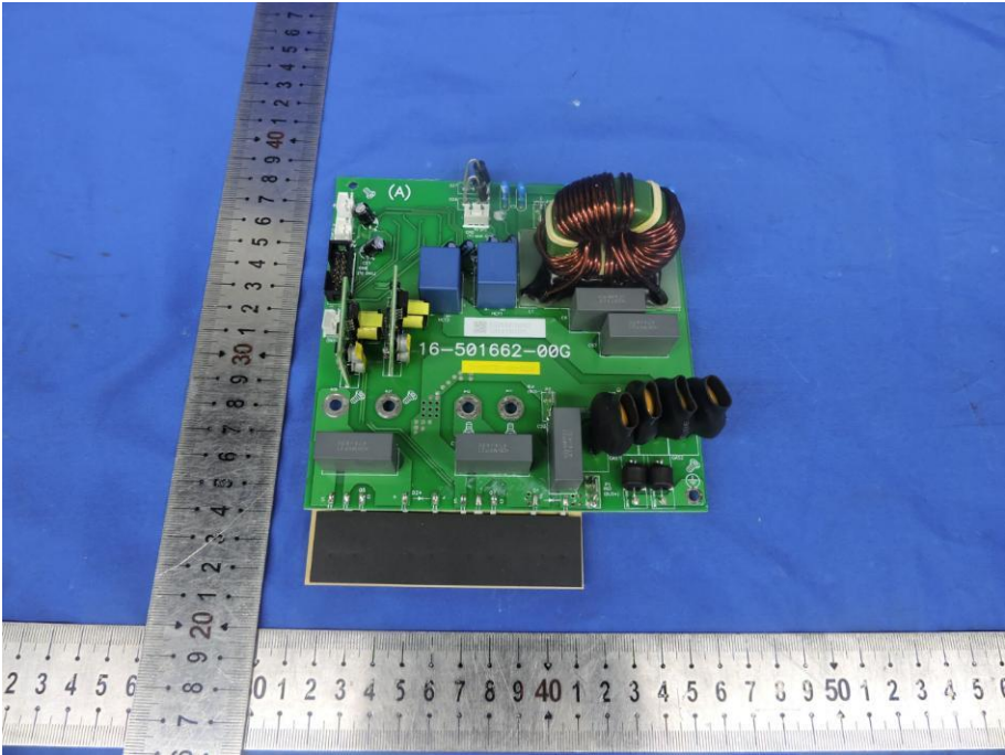
Fig. 17---PCB View
