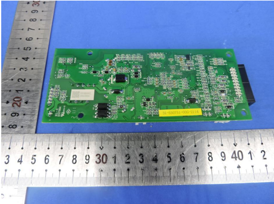
Fig. 16---PCB View
