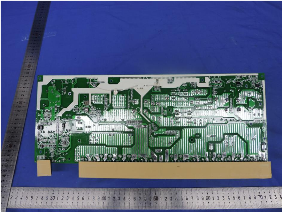
Fig. 22---PCB View
