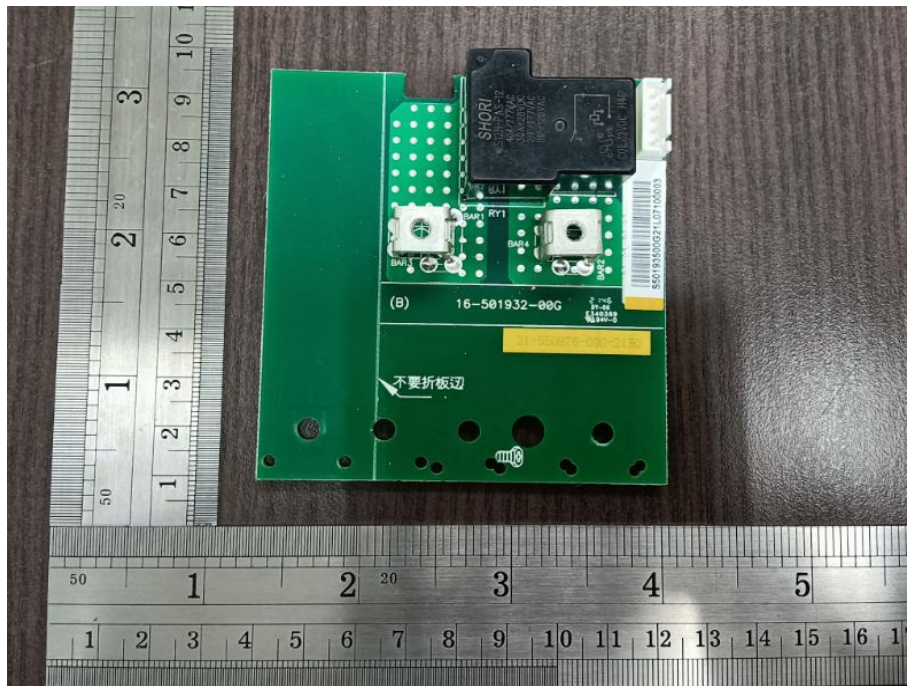
Fig. 31---PCB View
