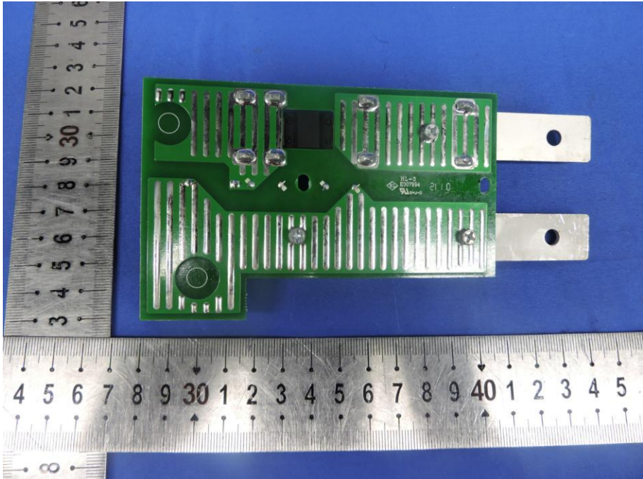
Fig. 24---PCB View
