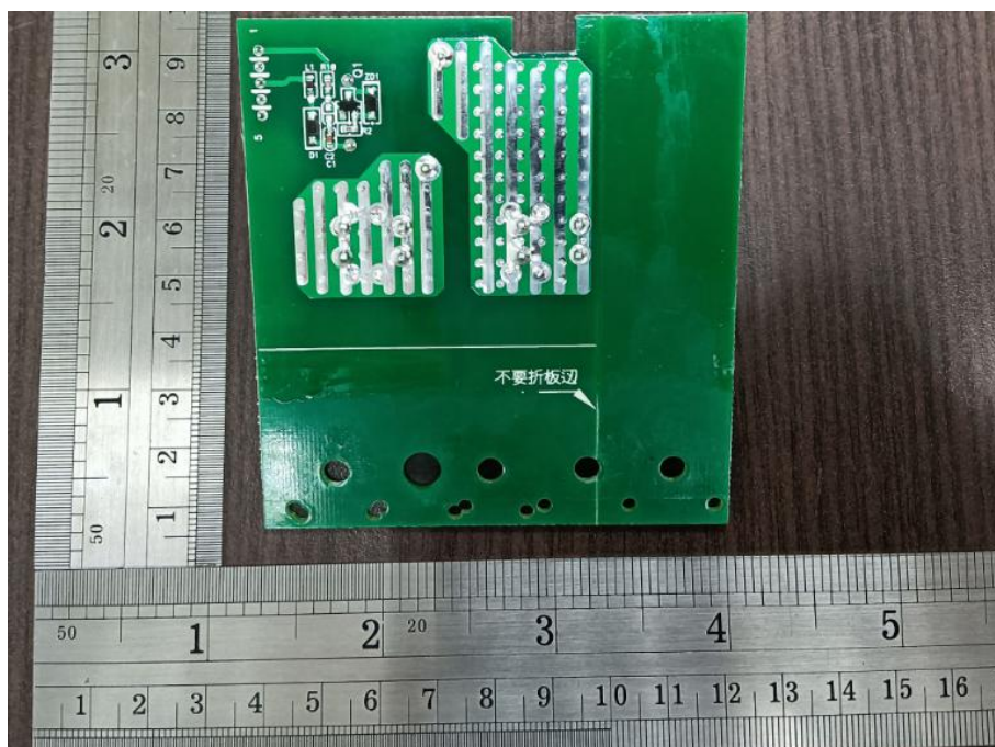
Fig. 32---PCB View
