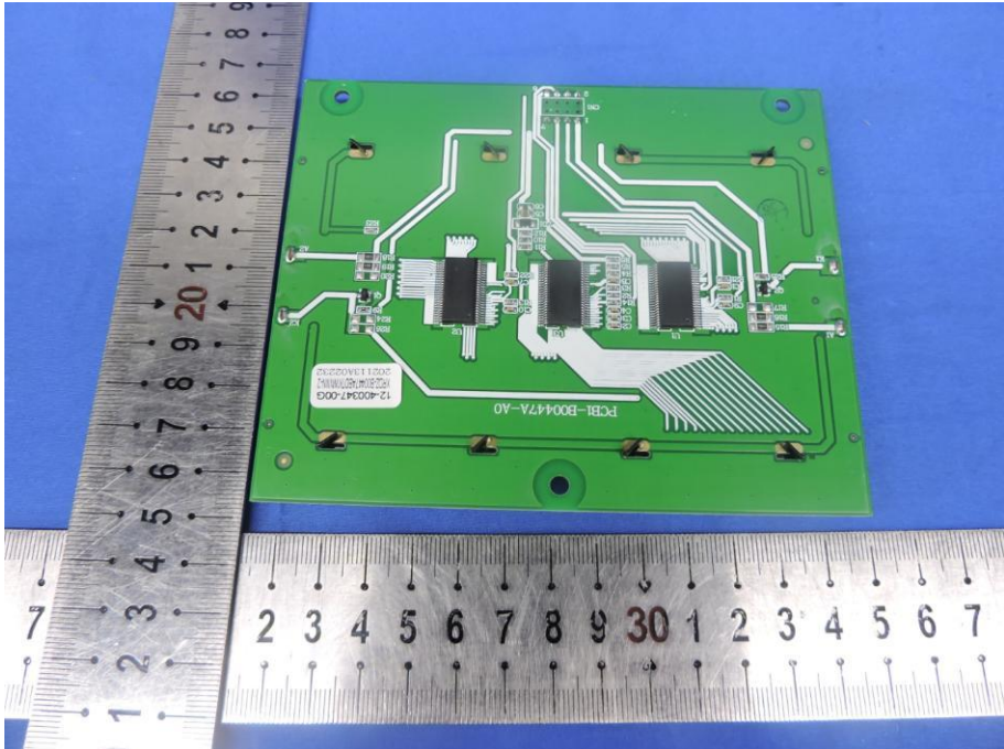
Fig. 8---PCB View
