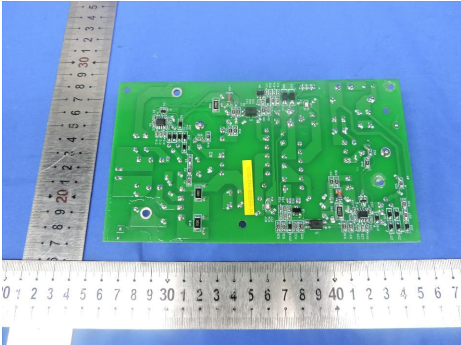
Fig. 14---PCB View
