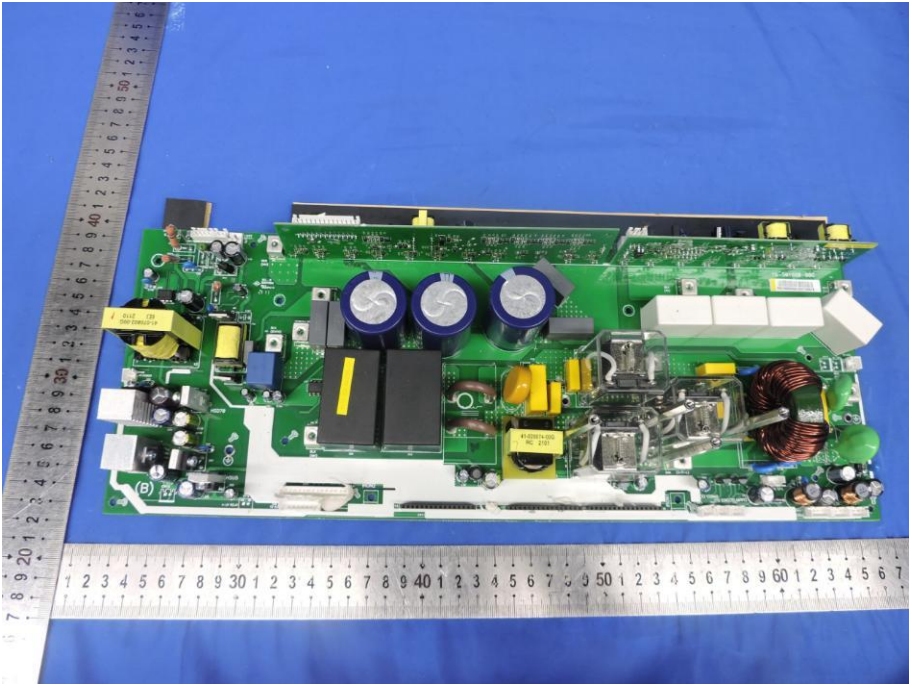
Fig. 21---PCB View
