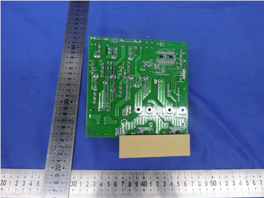
Fig. 18---PCB View
