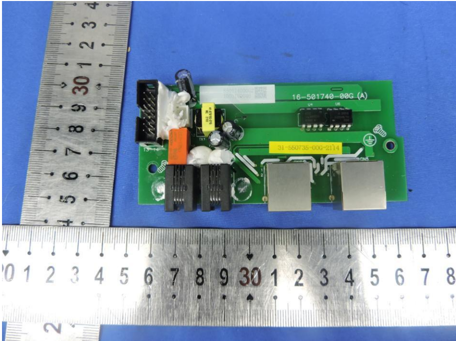
Fig. 29---PCB View
