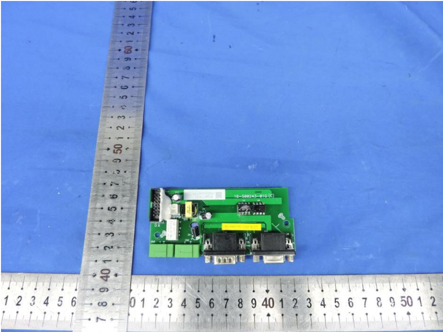
Fig. 17---PCB View
