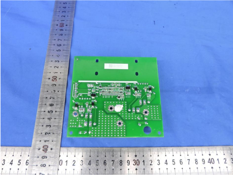
Fig. 14---PCB View
