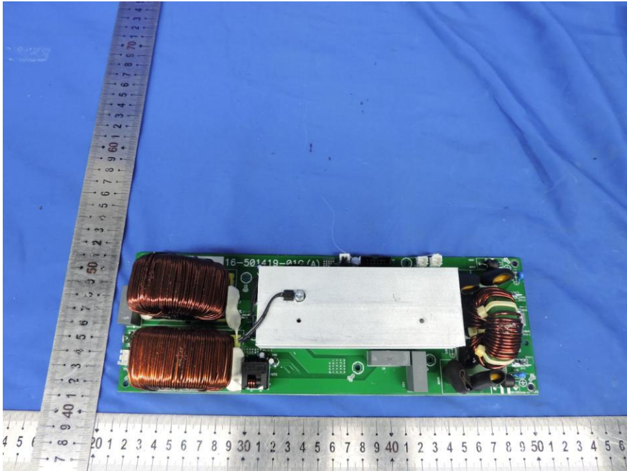
Fig. 9---PCB View
