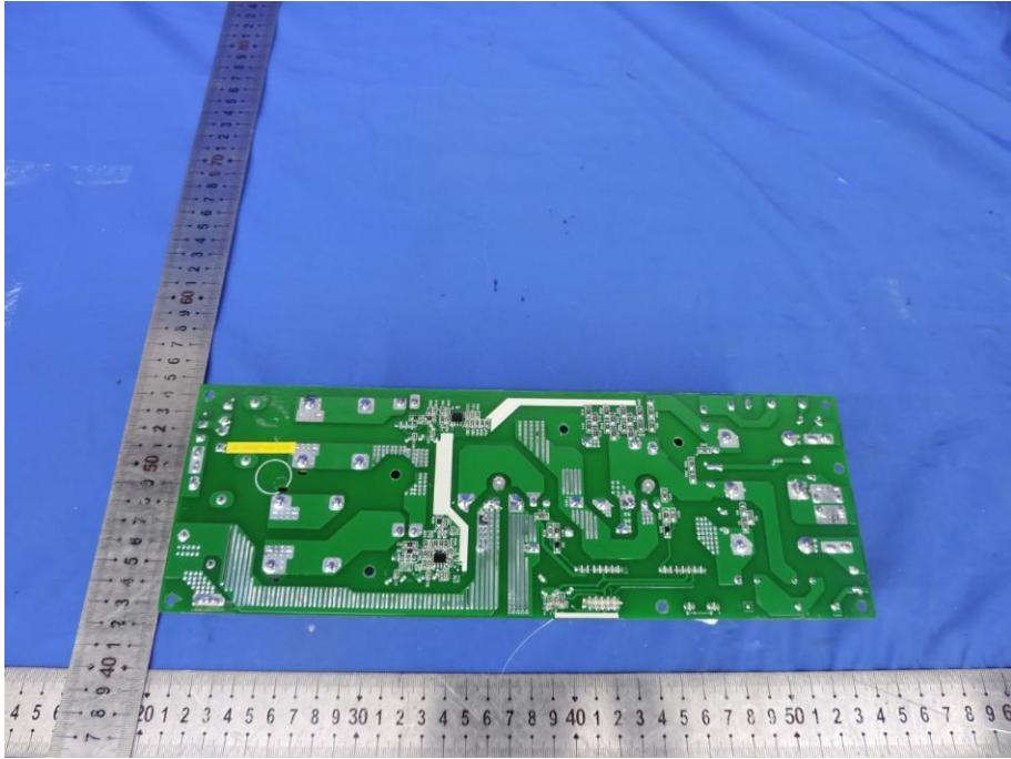
Fig. 10---PCB View
