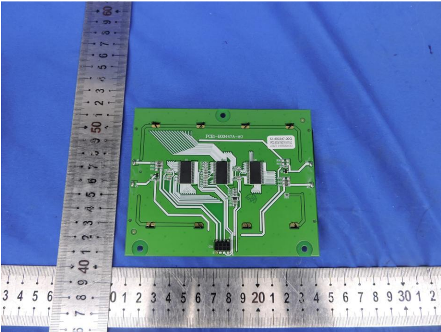
Fig. 26---PCB View
