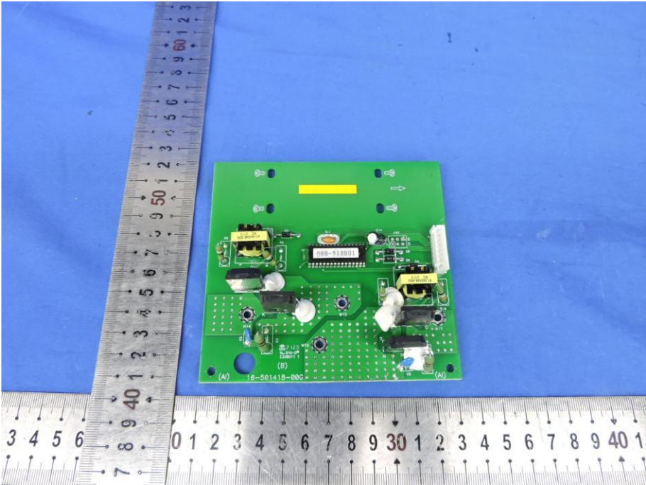
Fig. 13---PCB View
