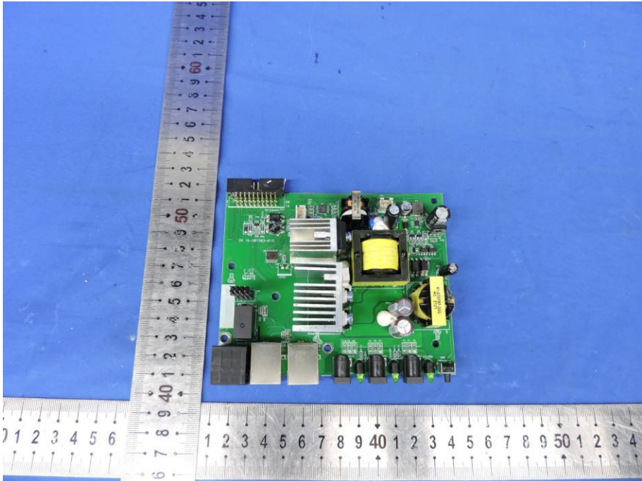
Fig. 19---PCB View
