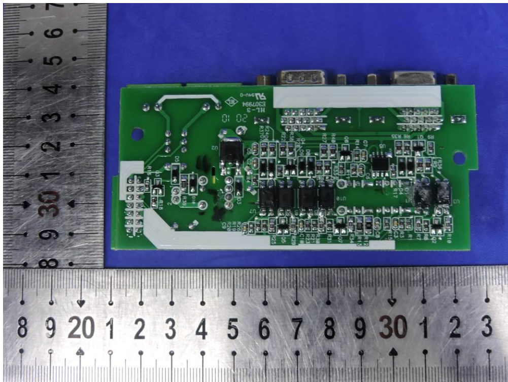
Fig. 15---PCB View
