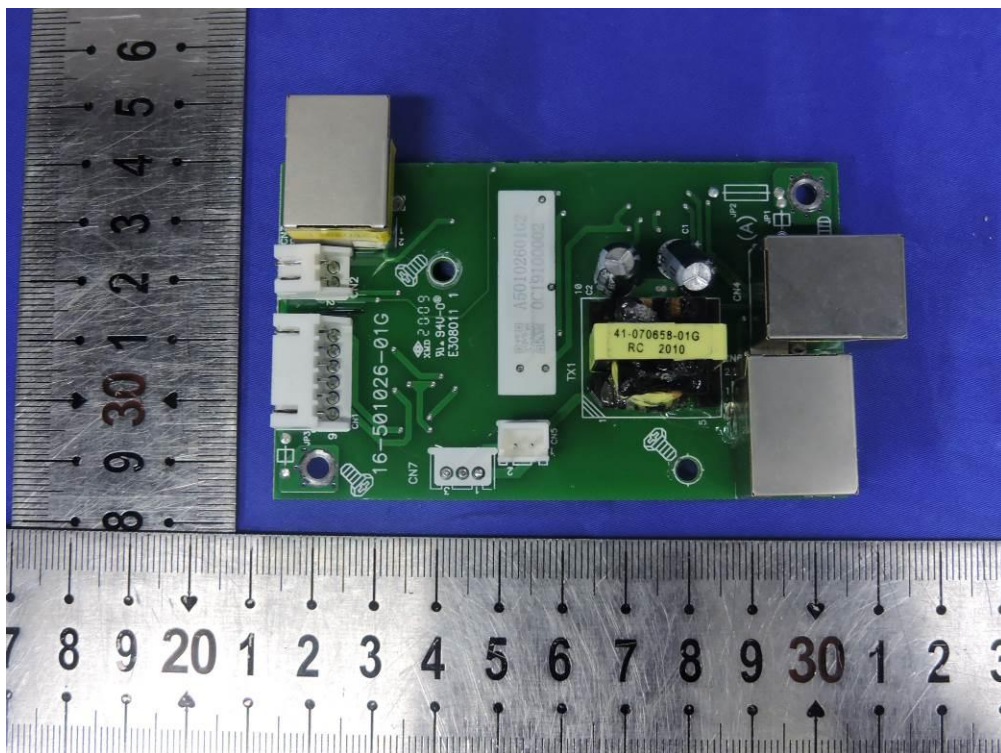
Fig. 16---PCB View
