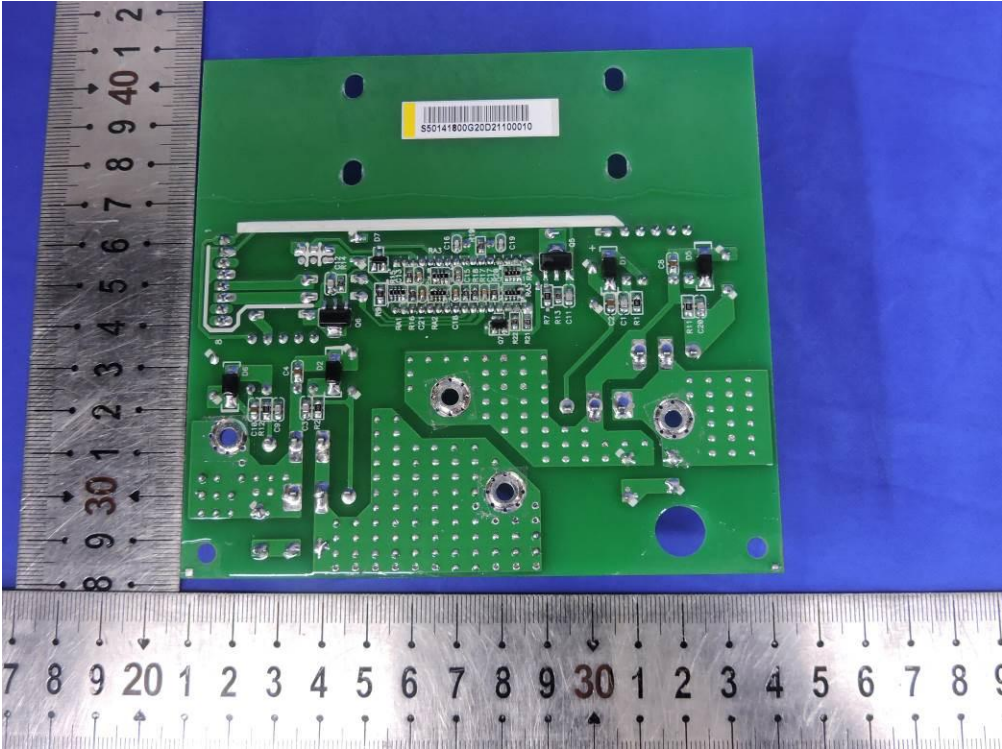
Fig. 9---PCB View
