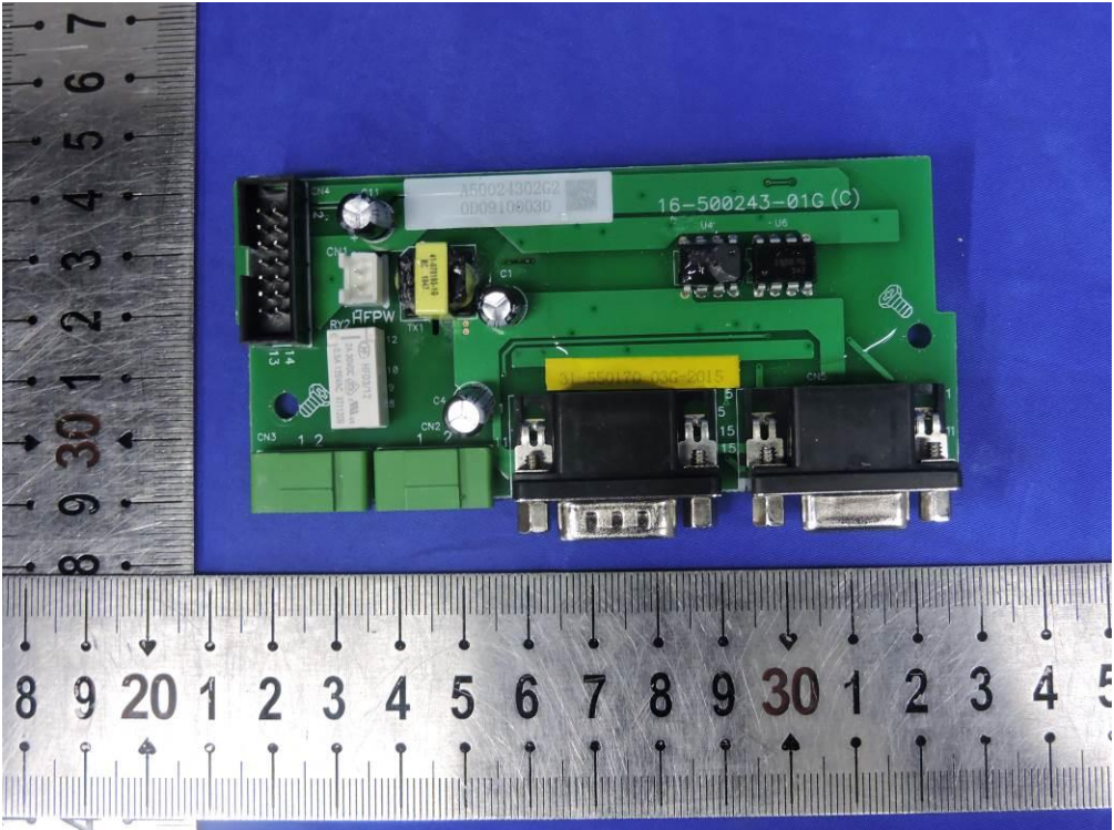
Fig. 14---PCB View
